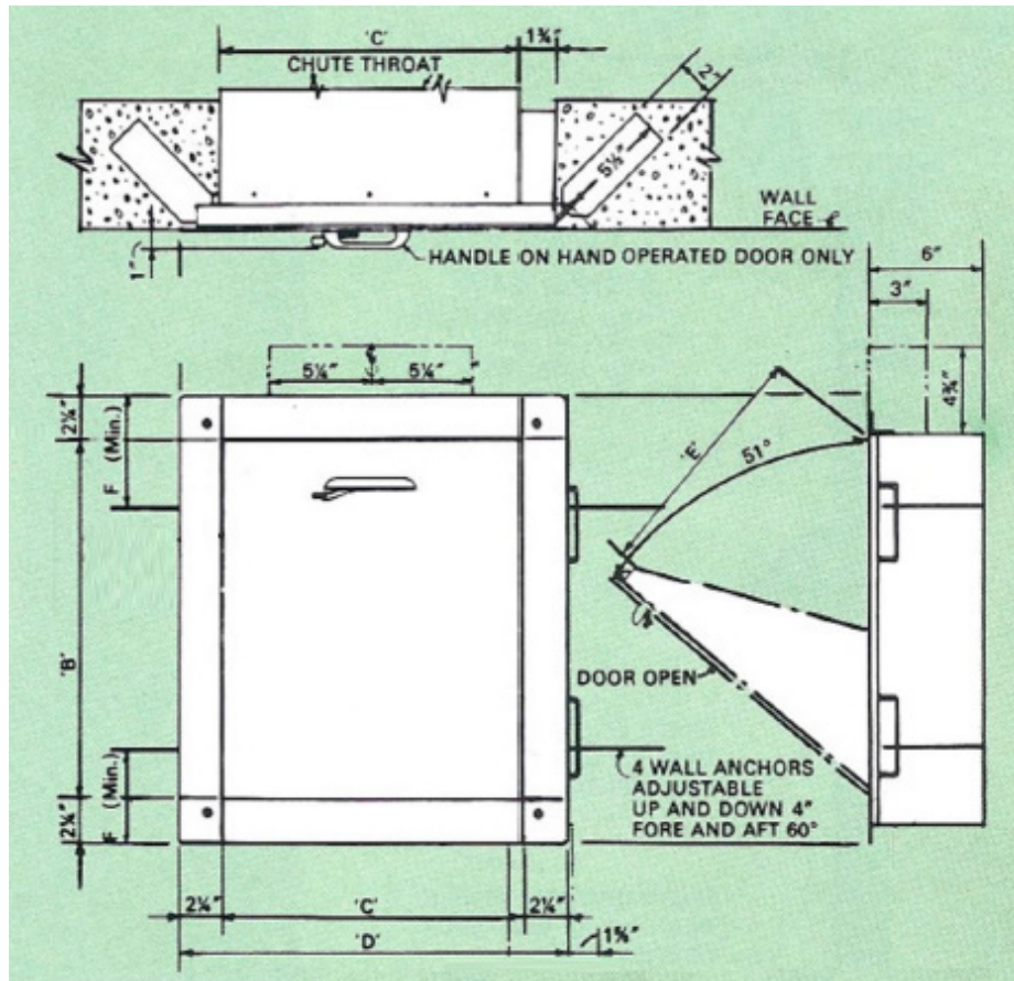
Wilkinson Style "Signature Series" Stainless Steel Trash Chute Door SKU: HWX09 DIMENSION CHART
