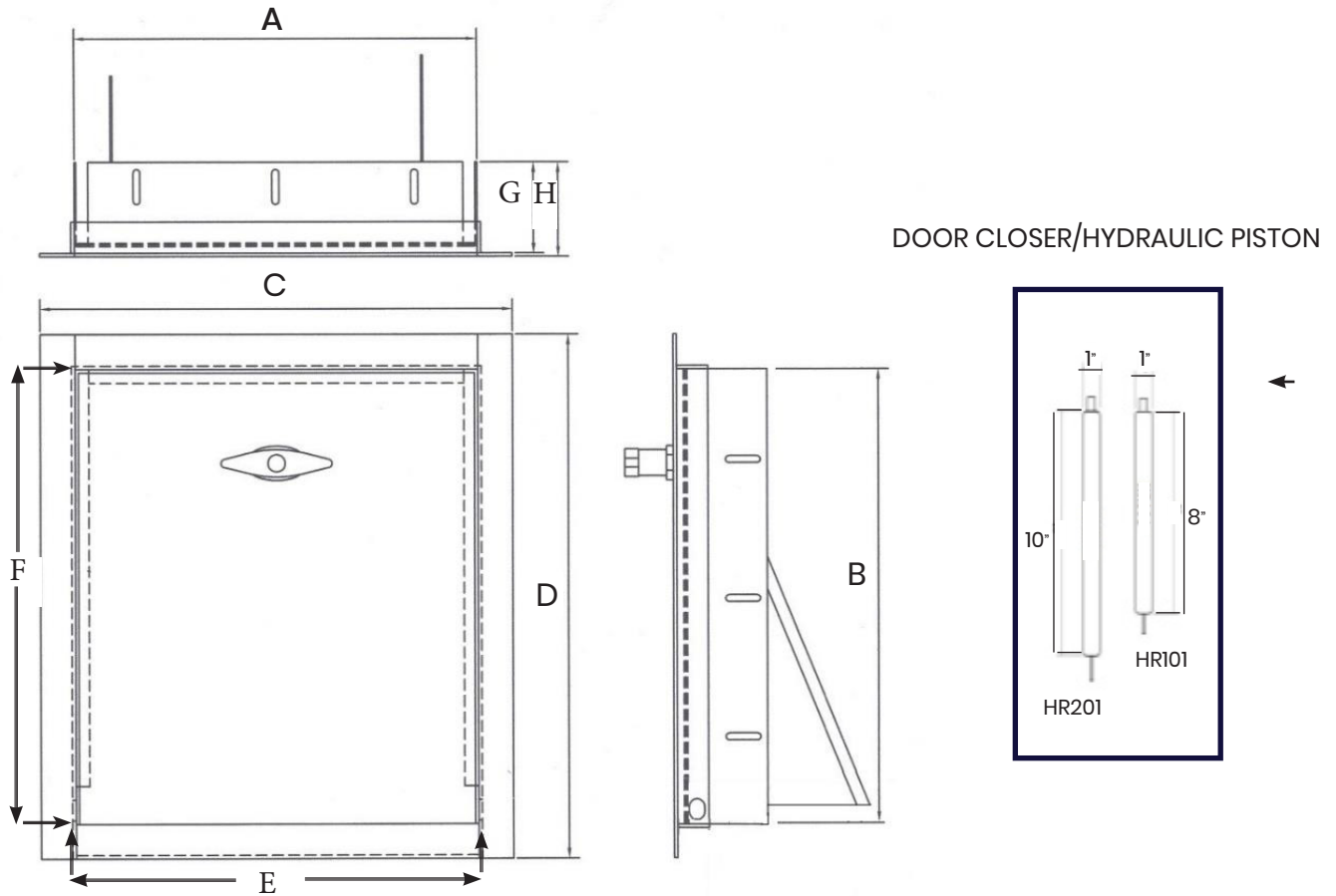
UNIVERSAL STAINLESS STEEL TRASH CHUTE DOOR SKU: HRX09 DIMENSION CHART (WITH CONNECTED TRIM – STANDARD WIDTH 2.25”)
